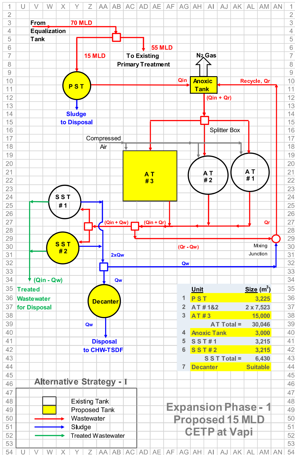
Figure 4.2: (Alternative Strategy - I) Process flow diagram of proposed 15 MLD for Expansion Phase -1 of CETP at Vapi. Here the conventional secondary settling tanks are used for solid-liquid separation.
